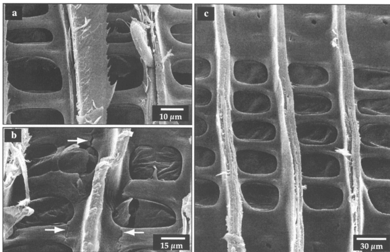
Fig. 8. a,b Cross-field pits between ray parenchyma and longitudinal tracheids initially impregnated to 105% increase in weight. Note the cracks in the cell walls of the tracheids ( arrows ). c Crossfield pits are from an unimpregnated specimen
