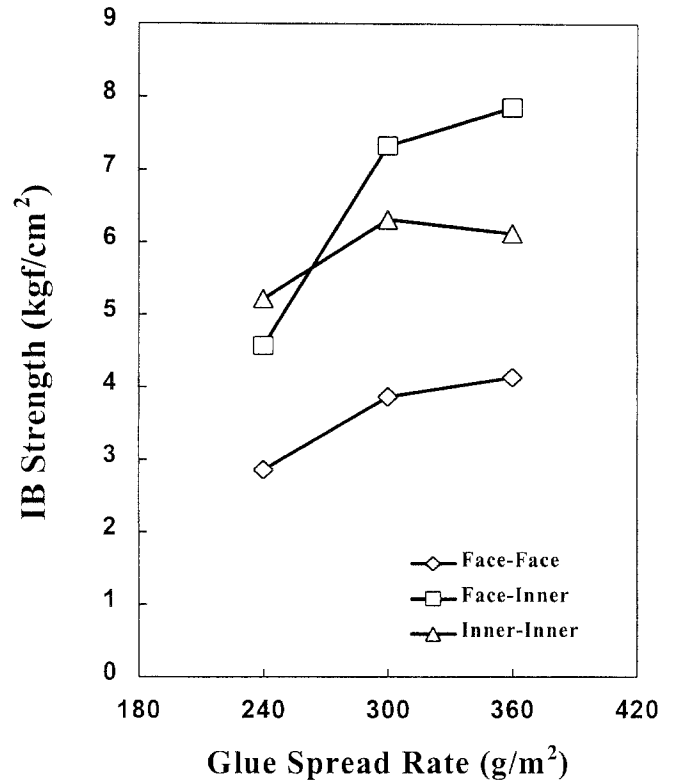
Fig. 4. Internal bond strength (IB) of two-ply LBL at different glue spread rates. Diamonds, glue spread rate on face-to-face layer; squares, glue spread rate on face to inner layer; triangles, glue spread rate on inner to inner layer
