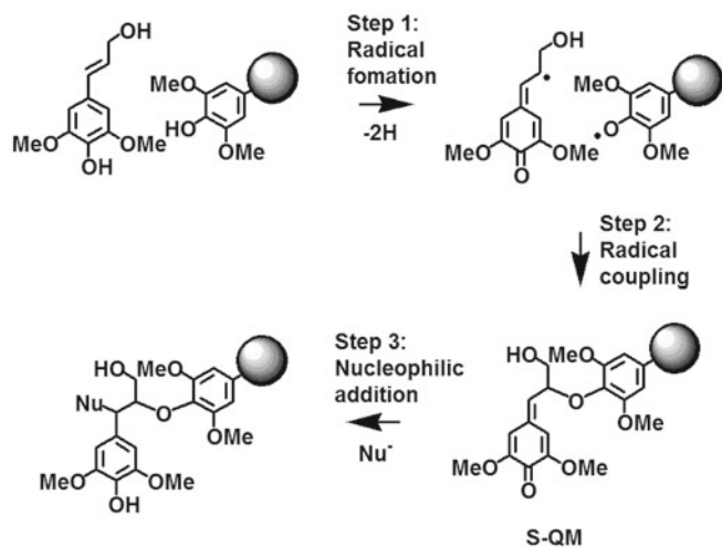
Fig. 1. Dehydrogenative polymerization of sinapyl alcohol (S-alc) via \beta -O-4 couplings
