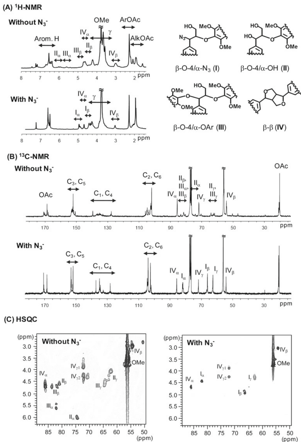
Fig. 7. Nuclear magnetic resonance (NMR) characterizations of acetylated S-DHPs from S-alc synthesized in the presence of azide ion. A ^1\text{H} -NMR spectra. B ^{13}\text{C} -NMR spectra. C 2D-heteronuclear single quantum coherence (HSQC) spectra
