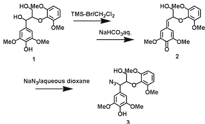
Fig. 8. Synthetic scheme for model compound 3. TMS, trimethylsilyl
