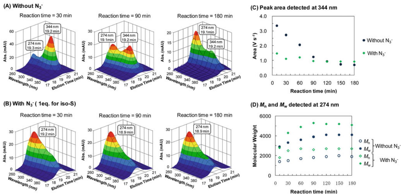
Fig. 5. Gel permeation chromatography with photodiode array detection (GPC-PDA) monitoring of HRP-catalyzed polymerization of iso-S. A Three-dimensional (3D) PDA plots in polymerization without nucleophilic reagents. B 3D PDA plots in polymerization with azide ion
